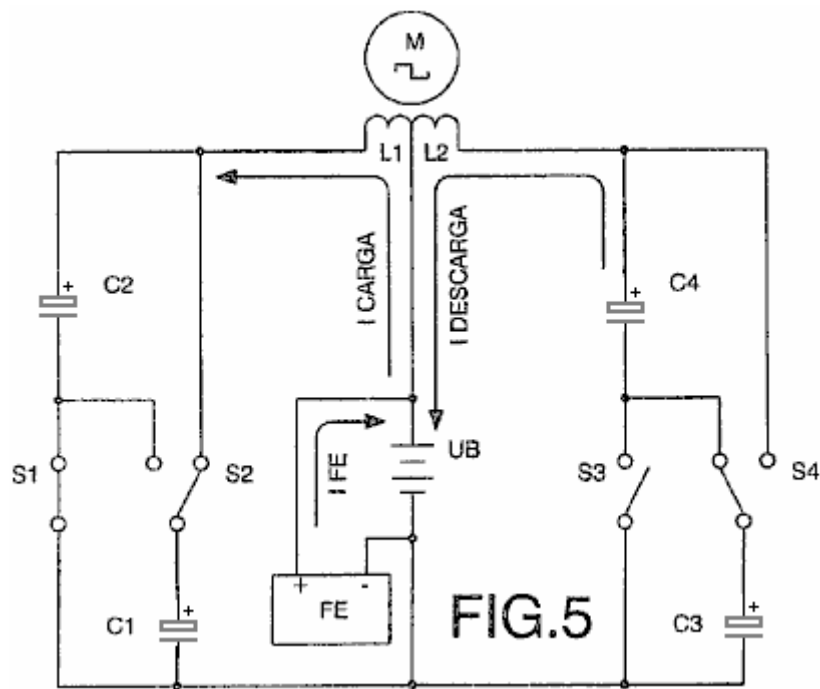
Fig.5 shows the electrical diagram of an alternating current motor with two windings connected between the battery and two pairs of capacitors.
