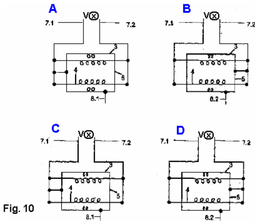
Fig.10 illustrates a circuit diagram of the electrical connection between the coils 3 and 4 in sets A, B, C and D. It can be seen that the sets A, B, C and D are enclosed between the coils 3 and their associated inductors or electromagnets 4. The supply conductors 7.1 and 7.2, of sets A, B, C and D must be interconnected. When feeding power to the coils 3 and 4 the phase should be connected to 7.1 and the neutral to 7.2.
