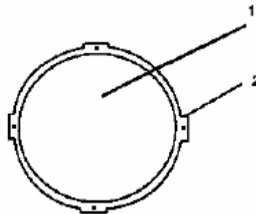
Fig.3 is a top view of one of the two hollow metallic hemispheres 1 which is part of the electron trap of free space proposed in this invention. Hemisphere 1 is preferably made from, but not limited to, aluminium, and it has mounting tabs 2.
