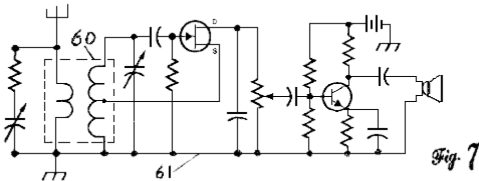
Fig.7 shows a view of a full-length transformer, used as an inductance in a radio receiver or other similar electronic circuit 61 . In this case the transmitter coil is between the aerial and ground, and the collector coil acts as the radio frequency inductance.
