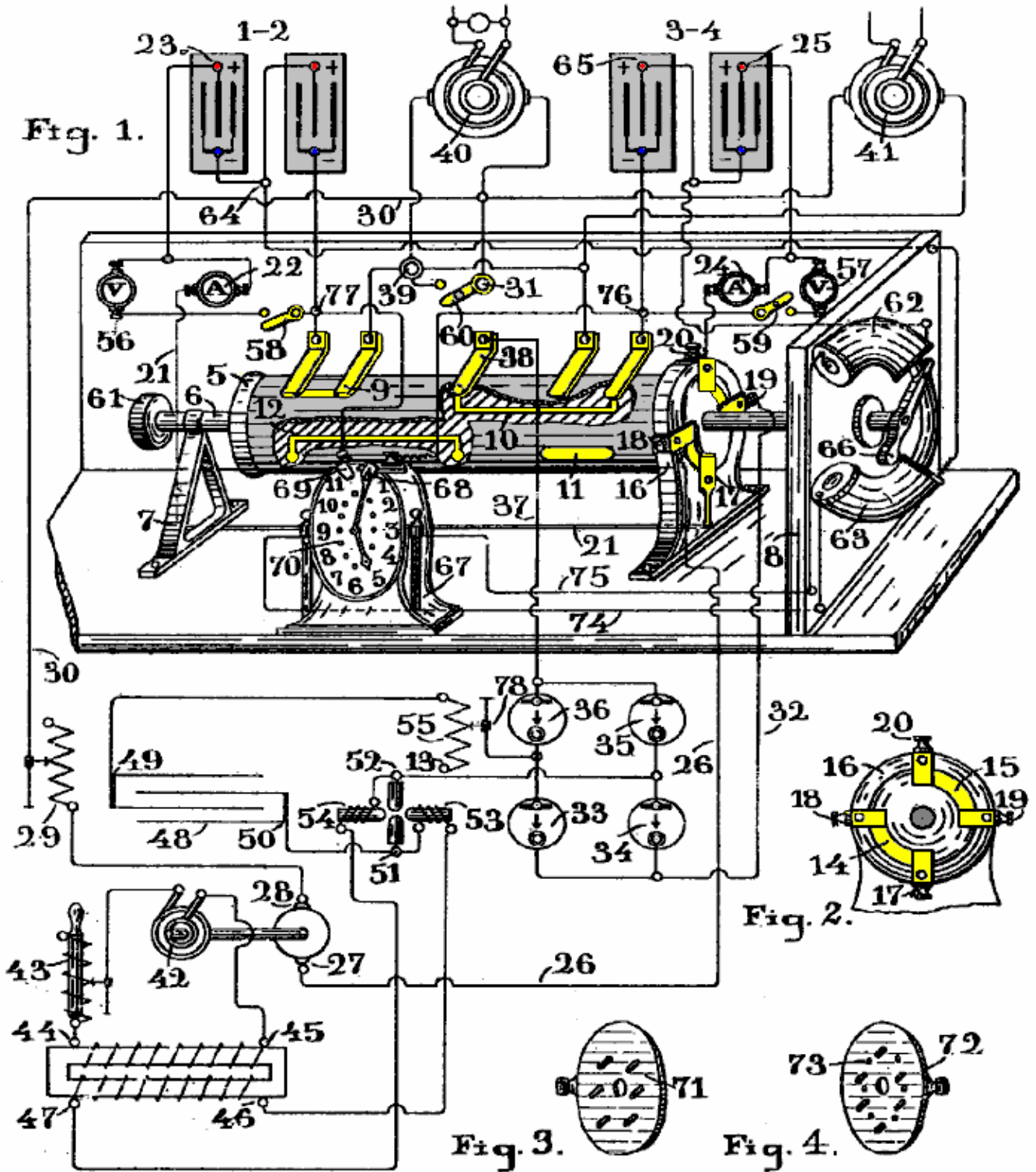
This circuit shows the circuit connections of the arrangement and a perspective view of a commutator. Figure 2 is a lateral view of a part of the same apparatus, and figures 3 and 4 are parts of the same machine, whose location and use will be explained later.
