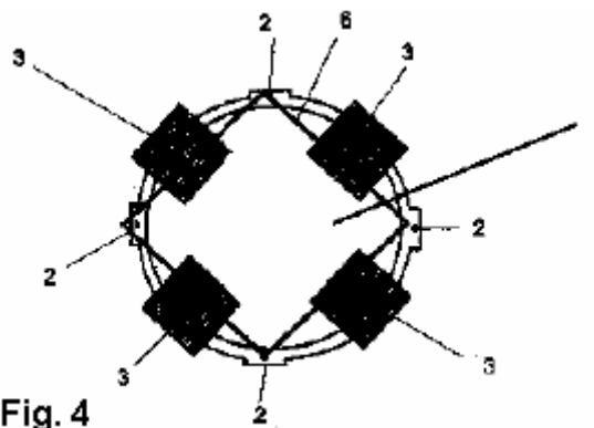
Fig.4 is a bottom view of metallic hemisphere 1. It has four electromagnetic field generating devices 3, positioned around the hemisphere and fixed to support 6 which is attached to hemisphere 1 by mounting tabs 2.
